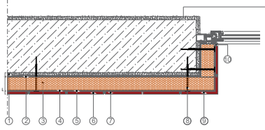
Yatay Kesit
