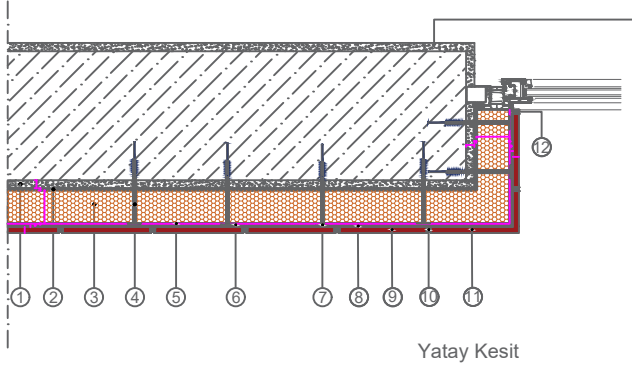
Yatay Kesit
