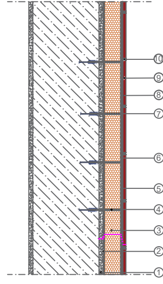
Yatay Kesit
